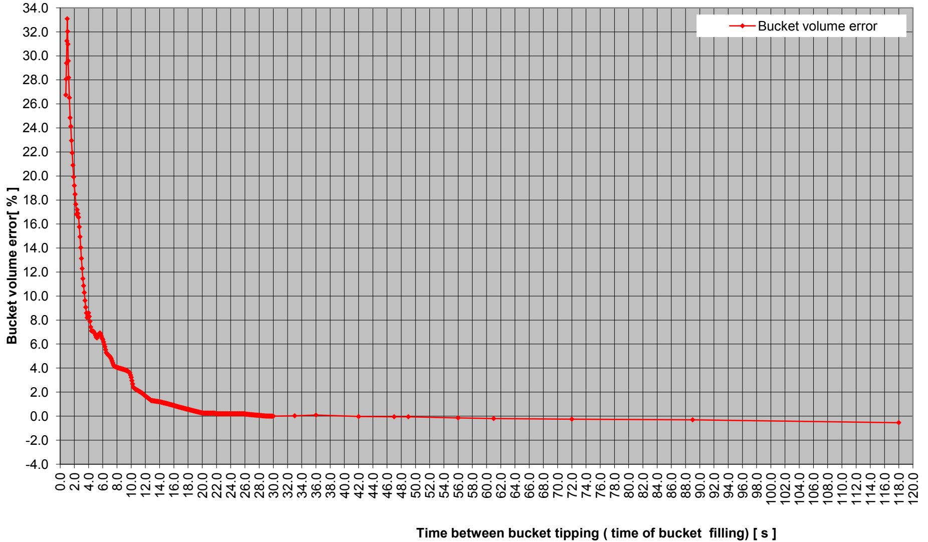
Dependence of the bucket volume error on tipping time ( time of bucket filling) for MR2(H)-01
